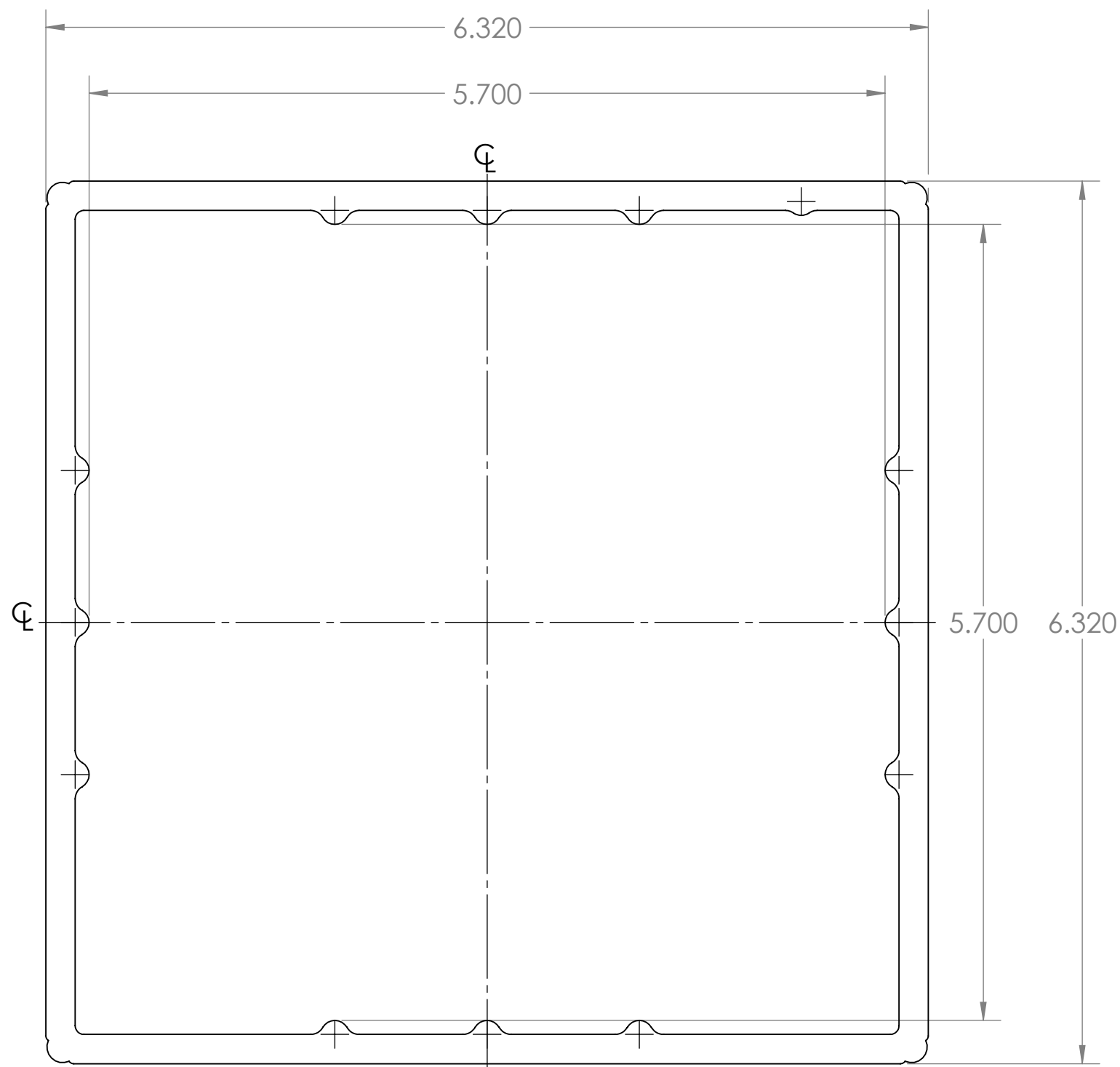
CROSS SECTION VIEW FOR CUSTOMER REQUIREMENT
