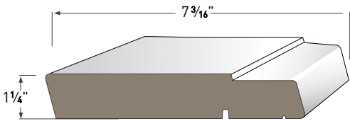
DOUBLE HUNG SILL AZM-7650 Length: 18'
