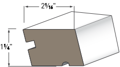
FARMHOUSE SILL AZM-7640 Length: 16'
