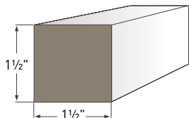
SQUARE PROFILE AZM-236 Length: 12'
