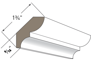
BED MOULDING AZM-75 Length: 16'
