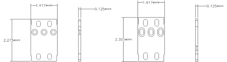
FIGURE 15 – LIBERTY RAIL BRACKETS
