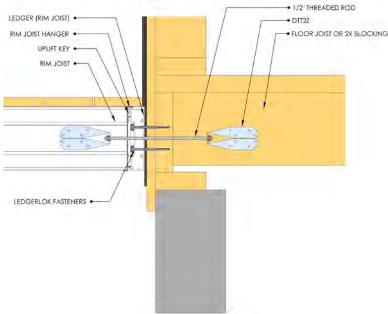
LEDGER CONNECTION DETAIL (THE LATERAL TENSION DEVICE)
