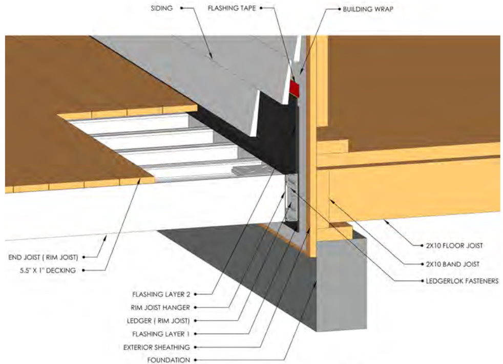
LEDGER CONNECTION DETAILS
