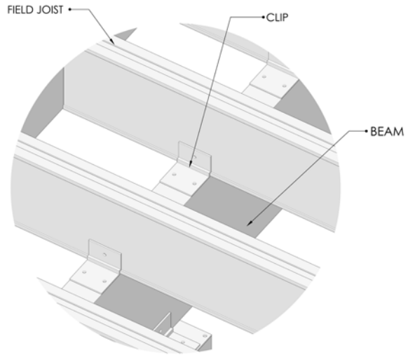
FIELD JOIST TO BEAM CLIP SCALE 1:4
