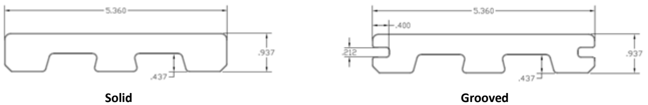
FIGURE 8 – CLASSIC, PRIME, PRIME + SOLID & GROOVED DECK BOARD PROFILES
